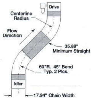
The illustration above shows the placement of straight sections between offsetting curves for a MultiSpan conveyor.
