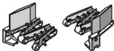
DS5220A-2/3 - LH 6MM RAISED / 30MM MSG 2/3 DS5240A-2/3 - RH 6MM RAISED / 30MM MSG 2/3
